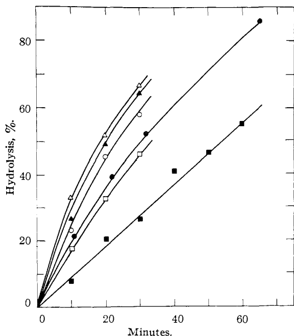
Fig. 1.—Relation between hydrolysis and time of incubation at 37^\circ and \text{pH } 7.0 . Substrate—acetyl-L-alanine at 0 , \bullet , 1 \times 10^{-4} M \circ , 1 \times 10^{-3} M \Delta , 1 \times 10^{-2} M \blacktriangle and 4 \times 10^{-2} M \square concentrations of \text{Co}^{++} added. Substrate—acetyl-L-capryline \blacksquare with no added \text{Co}^{++} . Concentration of substrate 0.017 M , temperature 37^\circ , 0.01 mg. protein N in each digest.
