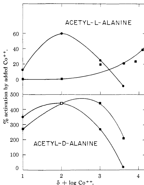
Fig. 2.—Relation between activation by cobalt and substrate concentration. Substrate concentration 0.017 M \bullet ; 0.167 M \blacksquare , \text{pH } 7.0 , temperature 37^\circ . Acetyl L-alanine, 0.01 mg. protein N in each digest; acetyl D-alanine, 1 mg. protein N in each digest.
